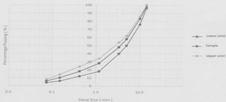
Percentage Passing vs Sieve Size
